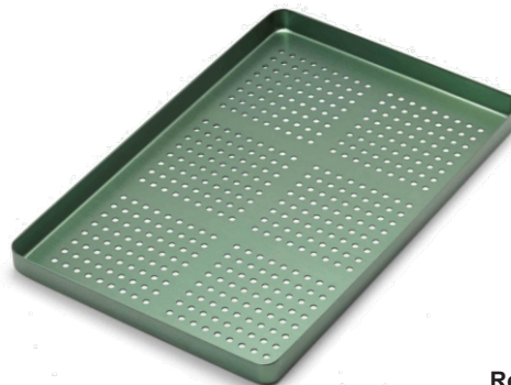
Small Tray Perforated 185 x 140 x 15mm
